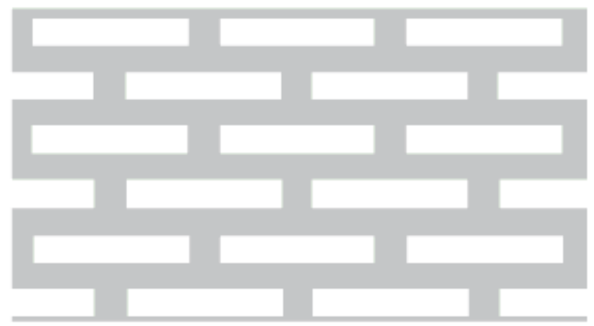
3,5 x 20mm - AL c = 7,0mm C = 24mm AA 41%
